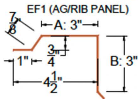
GABLE RAKE
