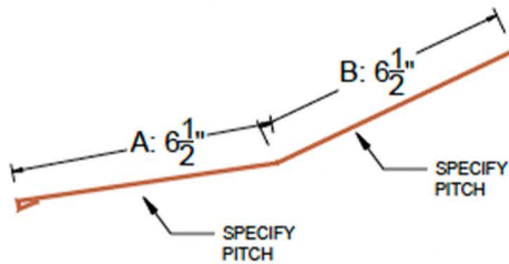
TRANSITION TF7 (STANDING SEAM PANEL)
