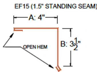
GABLE RAKE
