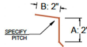
EAVE DRIP (2X2) ED4 (ALL PROFILES)
