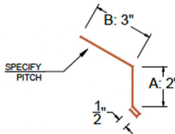
EAVE DRIP ED8 (STANDING SEAM)
