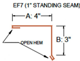
GABLE RAKE
