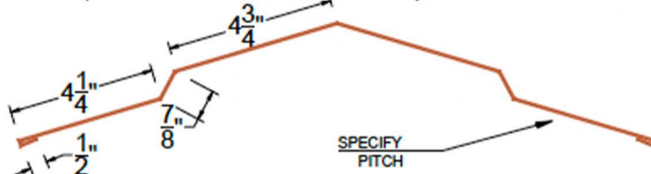
RIDGE CAP RC18 (FOR EXPOSED FASTENER PANEL)
