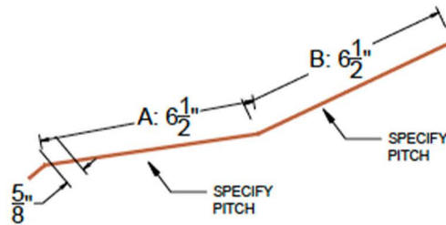
TRANSITION TF4 (EXPOSED FASTENER PANEL)
