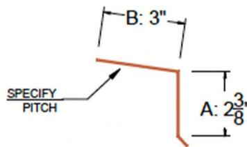
EAVE DRIP ED3 (ALL PROFILES)
