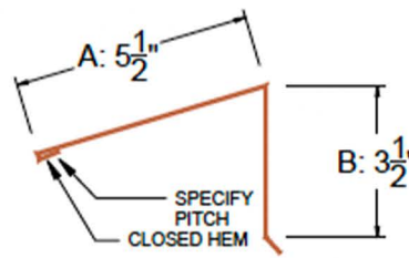
HIGH SIDE CAP HS5 (FOR PBR PANEL)
