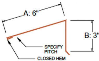
HIGH SIDE CAP HS1 (FOR RIB/AG PANEL)
