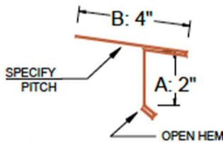
EAVE DRIP (BULLNOSE) ED7 (STANDING SEAM)
