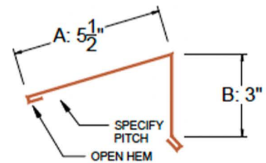
HIGH SIDE CAP HS7 (FOR 1" STANDING SEAM)
