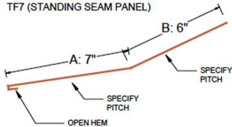
VALLEY
