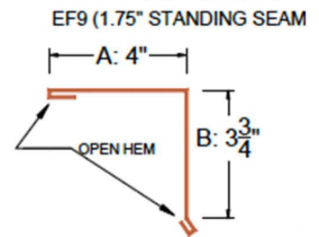
GABLE RAKE
