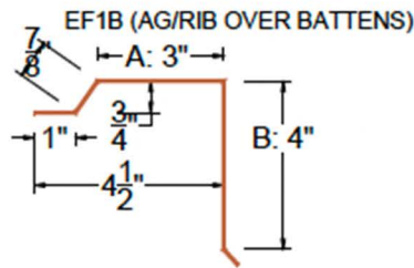
GABLE RAKE
