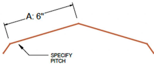
RIDGE CAP RC18 (FOR EXPOSED FASTENER PANEL)
