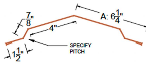
STANDARD RIDGE CAP RC2 (FOR EXPOSED FASTENER PANEL)
