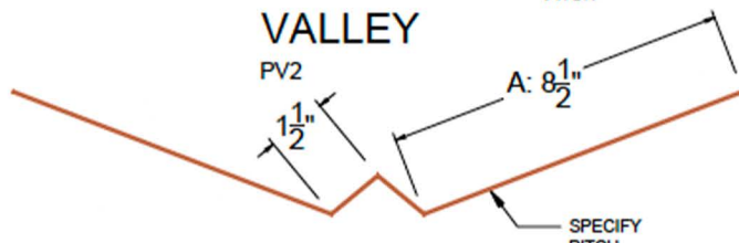
VALLEY (HEMMED)
