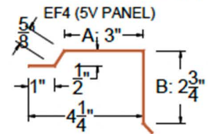
GABLE RAKE
