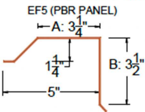
GABLE RAKE
