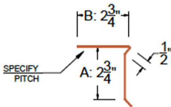
EAVE DRIP (FHA STYLE) ED1 (FOR EXPOSED FASTENER OR SHINGLE)
