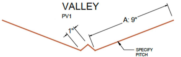
VALLEY
