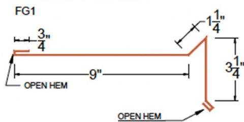
FLYING GABLE
