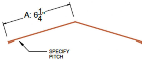
FLAT RIDGE CAP RC1 (FOR EXPOSED FASTENER PANEL)
