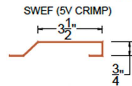
GABLE RAKE
