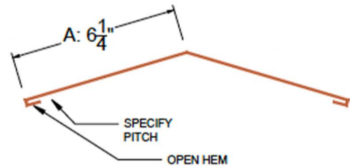
RIDGE CAP RC7 (FOR STANDING SEAM PANEL)
