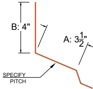
EW1 (EXPOSED FASTENER)
