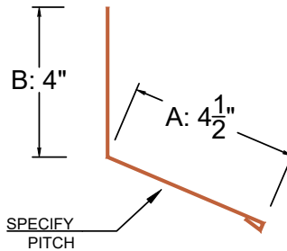
SW1 (AG/RIB PANEL)
