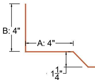
SW5 (PBR PANEL)
