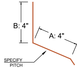
EW4 (EXPOSED FASTENER)
