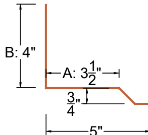
SW1 (AG/RIB PANEL)
