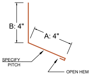
EW7 (STANDING SEAM)
